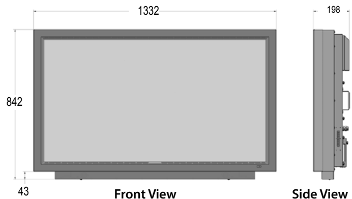
Dimensions with detachable speaker module. All measurements are in millimeters
